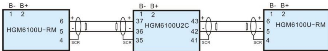
HGM6100U-RM and HGM6100U2C Typical Application Diagram
